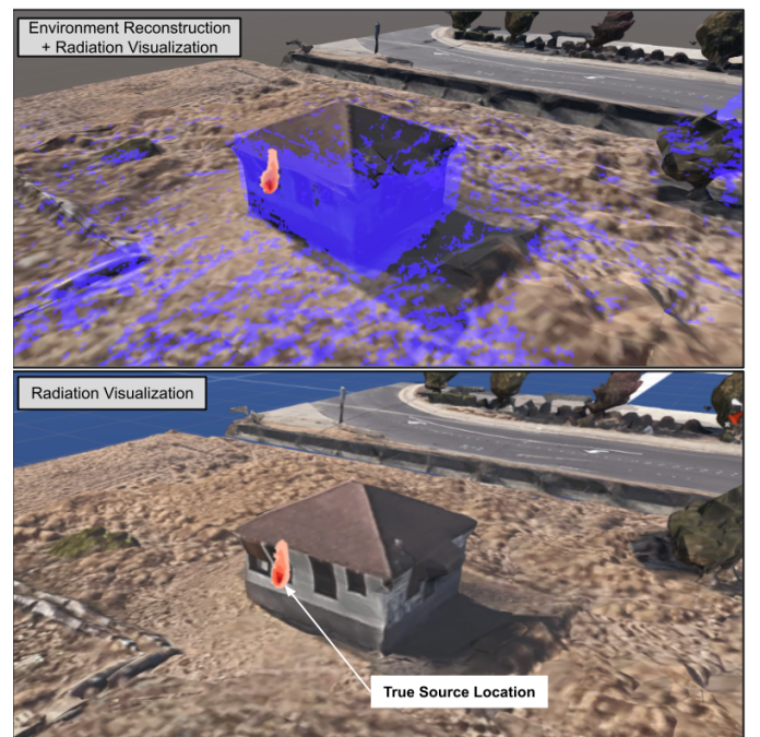
Fig. 8. Our system streams radiation and environment reconstruction data back to the VR interface, shown here, as colorized 3D meshes. The environment reconstruction (top, in purple) is generated by the LAMP's LiDAR and is used for the radiation reconstruction. We overlay the environment reconstruction on the baseline map to provide an accurate, real-time view of the sUAS's surroundings to the operator. The radiation-only visualization (bottom) shows reconstructed intensities of 662 keV reflecting measurements of the gamma-ray energies with the CLLBC-based NG-LAMP. Higher gamma-ray intensities are denoted by darker shades of red. Note we display only the 5 (of 6) most intense gamma-ray isosurfaces for visualization purposes. The operator can therefore intuitively localize the source to the darkest part of the mesh. For reference, the square building has a side length of about 8 meters.
